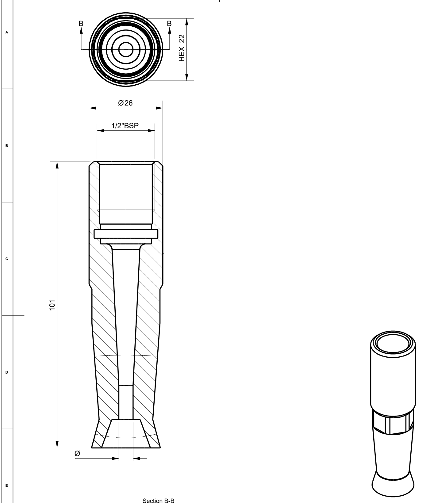
Section B-B
