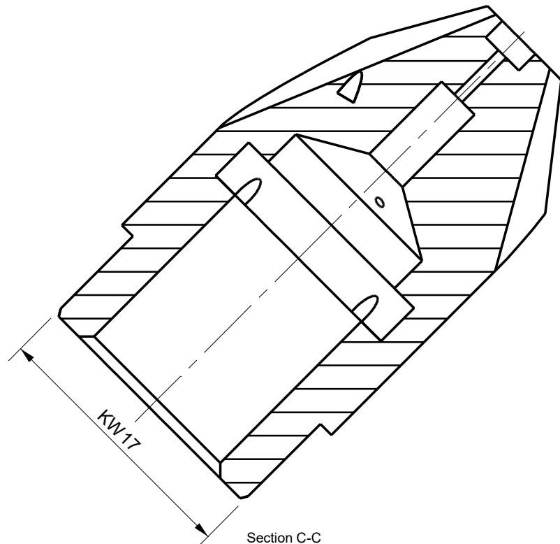
Section C-C
